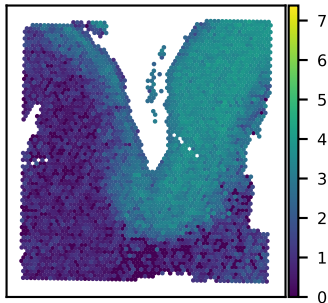
SNU51B SNAP25 expression Moran's I = 0.89
