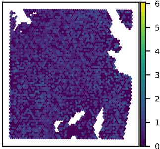
SNU51A ARHGAP23 expression Moran's I = 0.02
