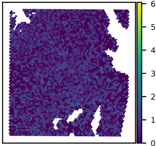
SNU51A PDRG1 expression Moran's I = 0.05
