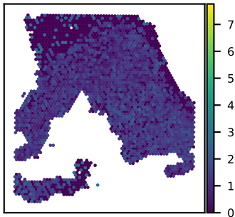
SNU18A MAP1LC3A expression Moran's I = 0.15
