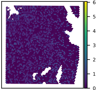
SNU51A ZNF766 expression Moran's I = 0.03
