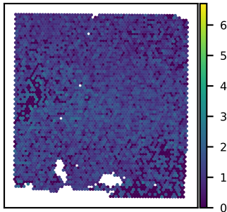
SNU43A PRELID3B expression Moran's I = 0.09
