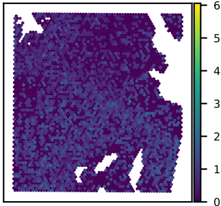
SNU51A HIST1H2BI expression Moran's I = 0.13
