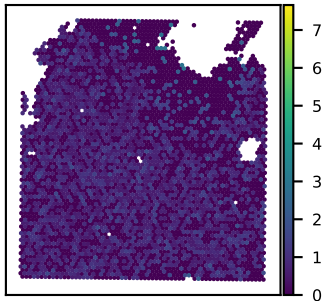
SNU21B GTF2B expression Moran's I = 0.04
