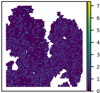
SNU27B TMEM150A expression Moran's I = 0.05
