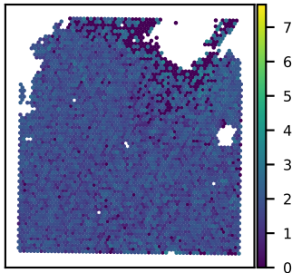
SNU21B HNRNPU expression Moran's I = 0.09
