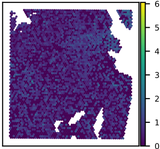
SNU51A SLC25A22 expression Moran's I = 0.08
