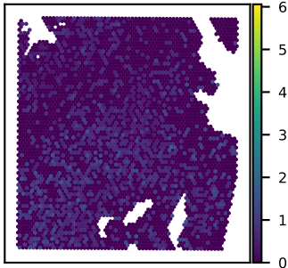
SNU51A ZNF804A expression Moran's I = 0.07
