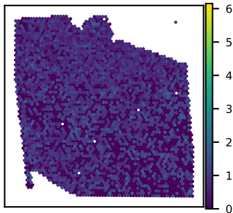
SNU27A GGNBP2 expression Moran's I = 0.02
