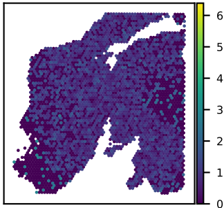
SNU24A VPS33A expression Moran's I = 0.05
