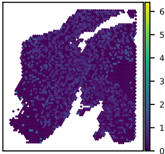
SNU24A TMEM150A expression Moran's I = 0.05
