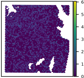
SNU51A CREB3L2 expression Moran's I = 0.03
