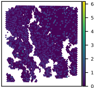
SNU16B EMILIN1 expression Moran's I = 0.05
