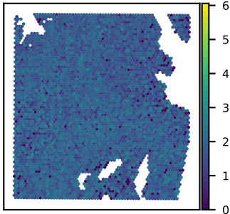
SNU51A GSTP1 expression Moran's I = 0.05
