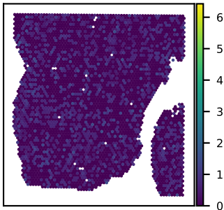
SNU25B RNF26 expression Moran's I = 0.01
