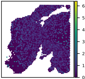
SNU24A TOPORS expression Moran's I = 0.03
