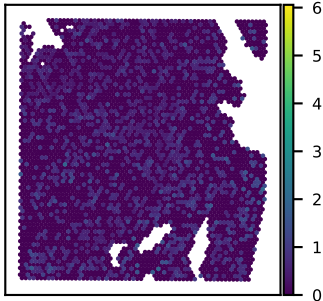
SNU51A PGBD1 expression Moran's I = 0.02
