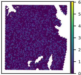
SNU51A PDIK1L expression Moran's I = 0.02
