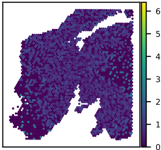
SNU24A RPAP2 expression Moran's I = 0.03
