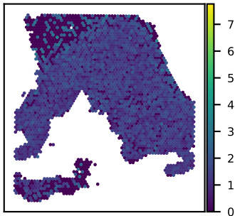
SNU18A FAM50A expression Moran's I = 0.14
