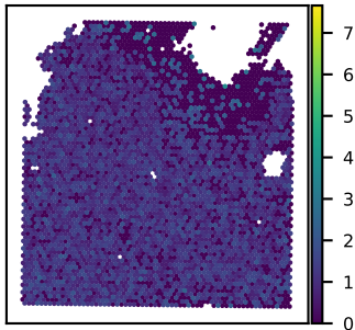
SNU21B ECHDC1 expression Moran's I = 0.10
