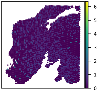
SNU24A HIST1H2BC expression Moran's I = 0.03
