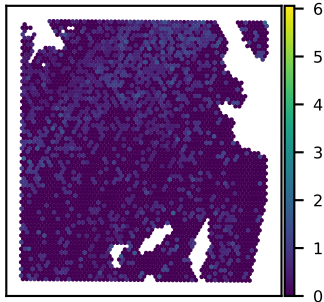
SNU51A CTSH expression Moran's I = 0.12
