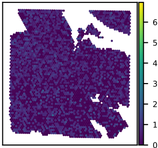
SNU24B CSNK1G3 expression Moran's I = 0.02
