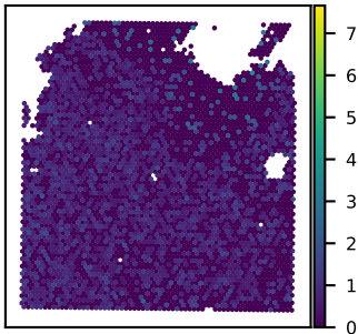
SNU21B SNRNP35 expression Moran's I = 0.04
