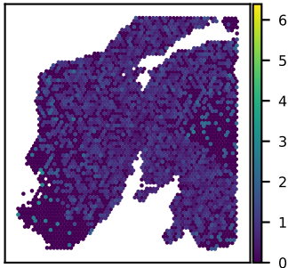
SNU24A INPP5B expression Moran's I = 0.05
