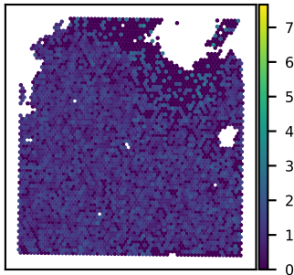
SNU21B LAMTOR3 expression Moran's I = 0.05
