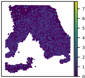
SNU18A SHARPIN expression Moran's I = 0.06
