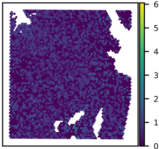
SNU51A GOLT1B expression Moran's I = 0.03
