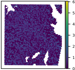
SNU51A SLC16A2 expression Moran's I = 0.02
