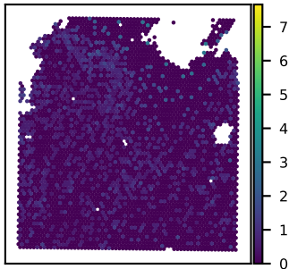
SNU21B HIST1H3A expression Moran's I = 0.06
