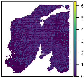
SNU24A MTPAP expression Moran's I = 0.04
