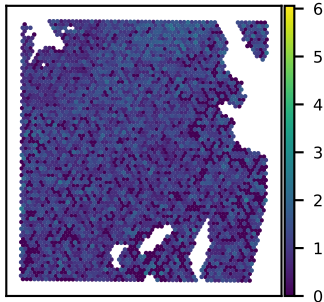
SNU51A PACS2 expression Moran's I = 0.06
