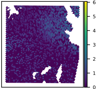
SNU51A SCG5 expression Moran's I = 0.28
