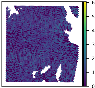
SNU51A MBOAT7 expression Moran's I = 0.03
