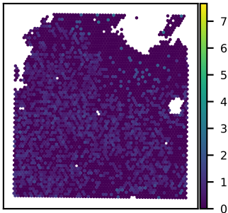
SNU21B NECTIN3 expression Moran's I = 0.07
