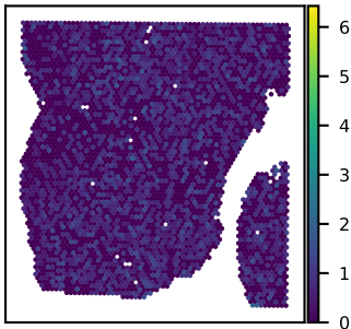
SNU25B SLC35G2 expression Moran's I = 0.01
