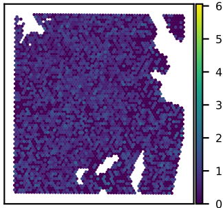
SNU51A TMEM168 expression Moran's I = 0.02
