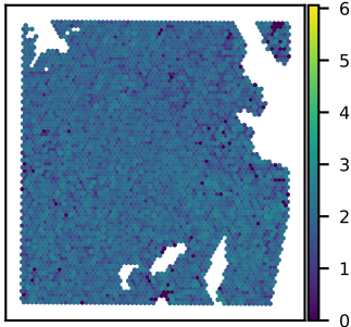
SNU51A SRRM2 expression Moran's I = 0.05
