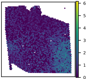
SNU27A RUNDC3A expression Moran's I = 0.43
