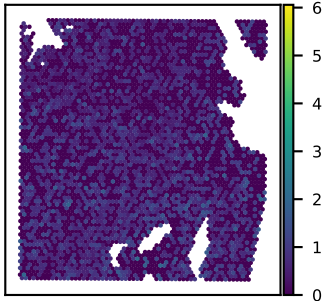
SNU51A SLC35E2A expression Moran's I = 0.02
