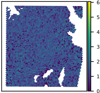
SNU51A POLR2I expression Moran's I = 0.02
