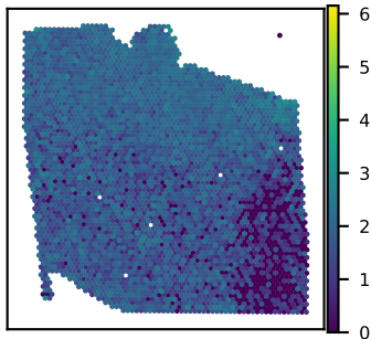
SNU27A IGFBP2 expression Moran's I = 0.44
