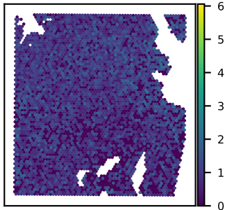
SNU51A PITPNB expression Moran's I = 0.06
