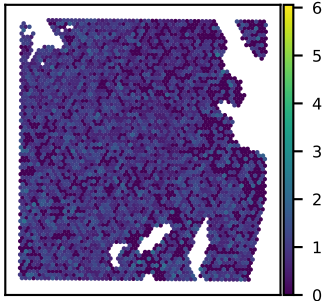
SNU51A NLGN2 expression Moran's I = 0.05
