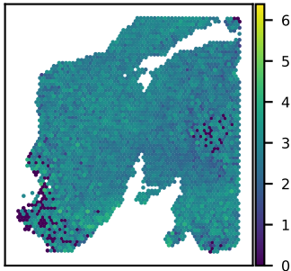
SNU24A SERPINA3 expression Moran's I = 0.19
